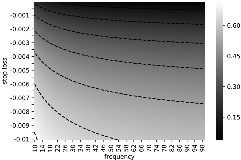
FIGURE 15.2 Heat-map of the implied precision as a function of n and \pi_- , where \pi_+ = 0.1 and \theta^* = 1.5
