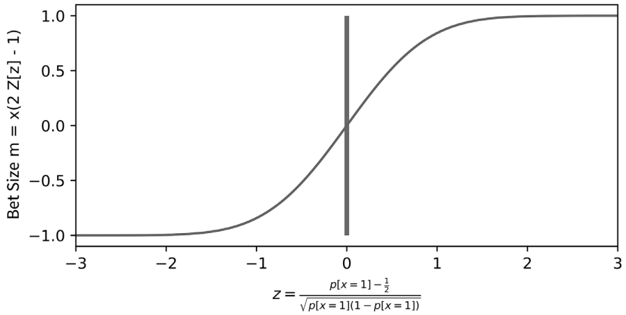
FIGURE 10.1 Bet size from predicted probabilities
