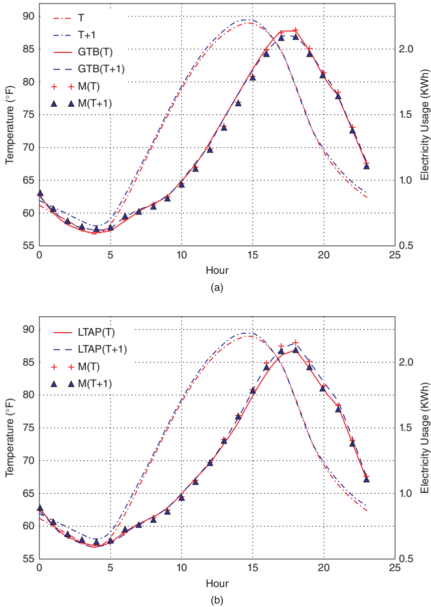
FIGURE 22.6 Gradient tree boosting (GBT) appears to follow recent usage too closely and therefore not able to predict the baseline usage as well as the newly develop method named LTAP. (a) GTB on Control group. (b) LTAP on Control group. (c) GTB on Passive group. (d) LTAP on Passive group. (e) GTB on Active group. (f) LTAP on Active group
