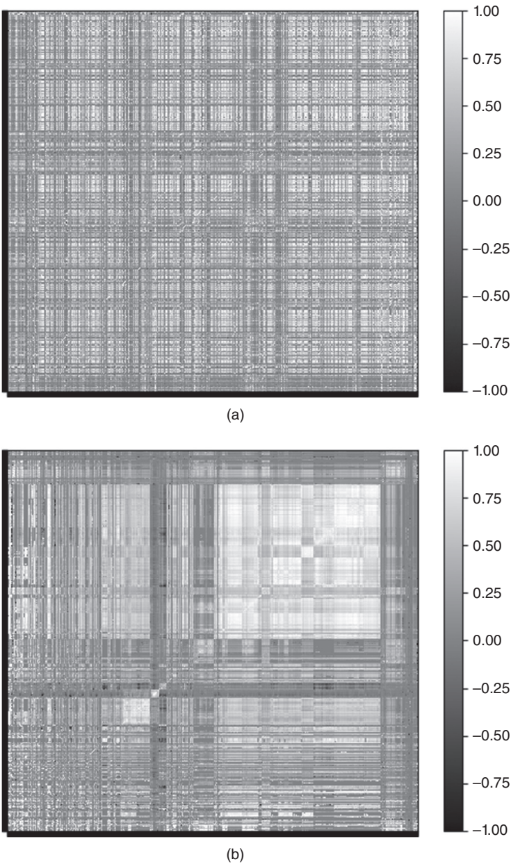
FIGURE 16.8 Correlation matrix before and after clustering The methodology described in this chapter can be applied to problems beyond optimization. For example, a PCA analysis of a large fixed income universe suffers the same drawbacks we described for CLA. Small-data techniques developed decades and centuries ago (factor models, regression analysis, econometrics) fail to recognize the hierarchical nature of financial big data.
