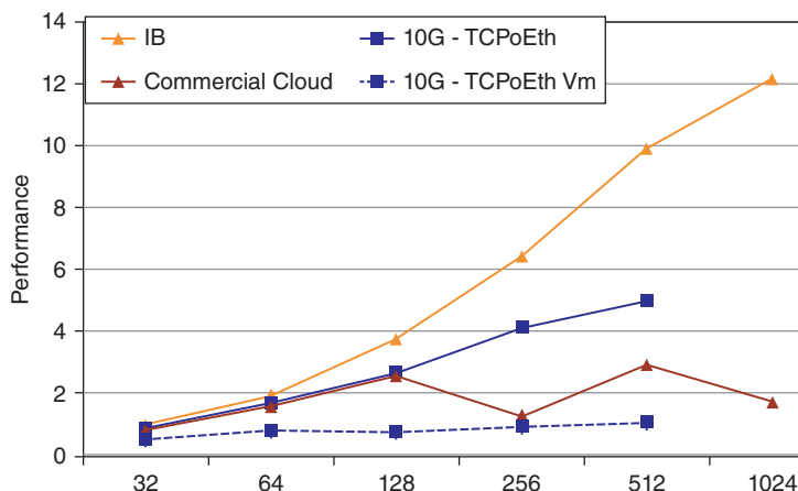
FIGURE 22.3 As the number of cores increases (horizontal axis), the virtualization overhead becomes much more significant (circa 2010)
