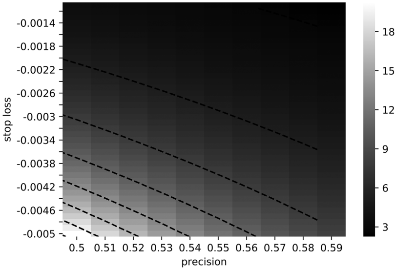
FIGURE 15.3 Implied frequency as a function of p and \pi_- , where \pi_+ = 0.1 and \theta^* = 1.5
